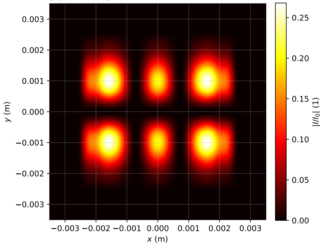
Intensity profile I(x, y, z = 3.503)/I_0 , P_{in}=0.5P_{cr} , artificial time
